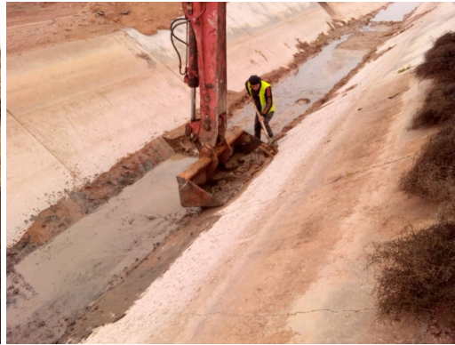
Above/ Below: Rehabilitation of the Maskaneh irrigation canal
